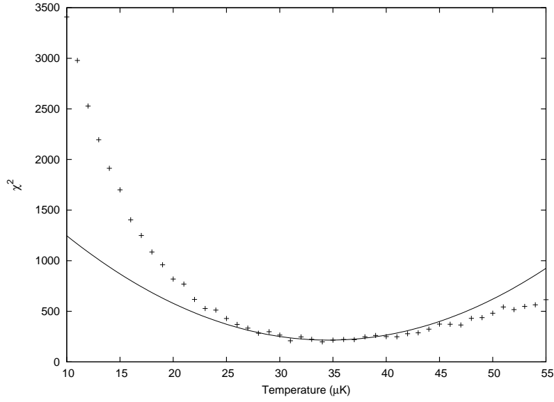
Figure 3.3: Plot of \chi^2 for different values of T used in the Monte-Carlo simulation (crosses). Fitting for T = 30 to 40 \mu\text{K} to a parabolic function (solid curve) yields \chi^2 = a * (T - T_o)^2 + c with a = 1.7(6) \mu\text{K}^{-2} , T_o = 34.6(5) \mu\text{K} , c = 215(8) . Errors in brackets reflect the error in fitting to a parabolic function.
